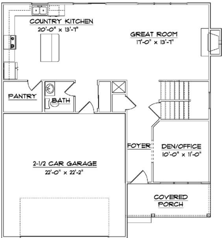
MAIN FLOOR - 948.1
