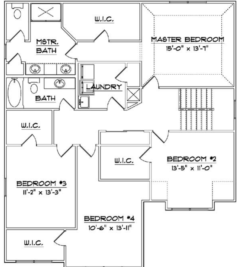
SECOND FLOOR PLAN - 1419.3
